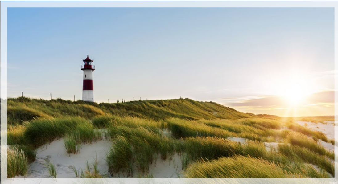
Fig. 7.1. Coastal sand dunes at Sylt, Germany (Photo: Michael Thaler/ Shutterstock).
